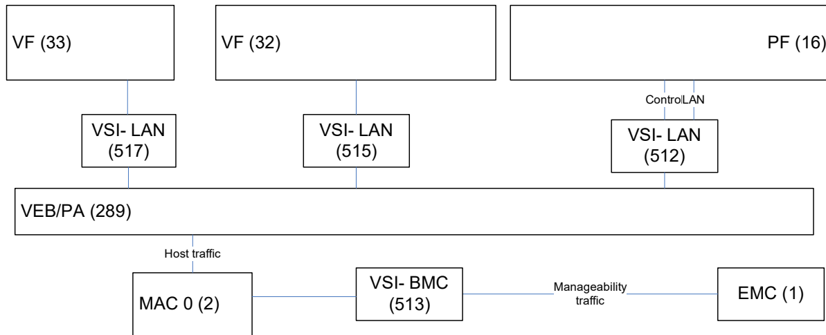
Figure 7-53. VEB/VEPA
